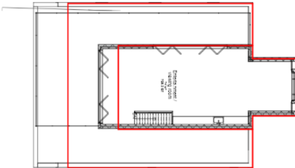
4 Second floor plan 1 : 100
